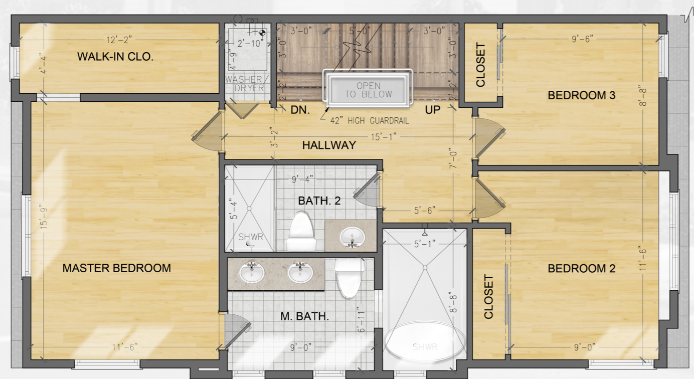
3 THIRD FLOOR PLAN EAST BUILDING
