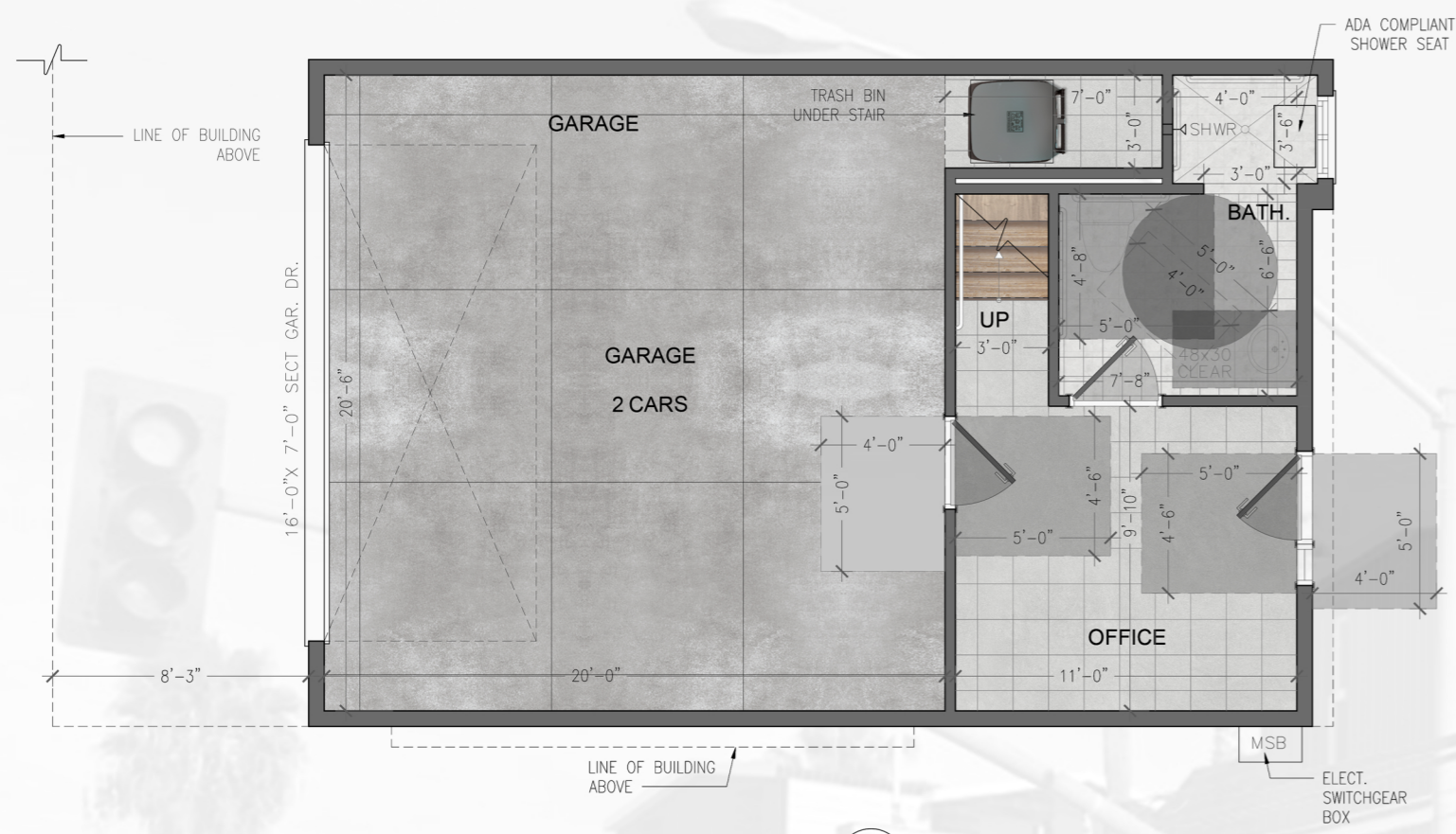
1 FIRST FLOOR PLAN EAST BUILDING
