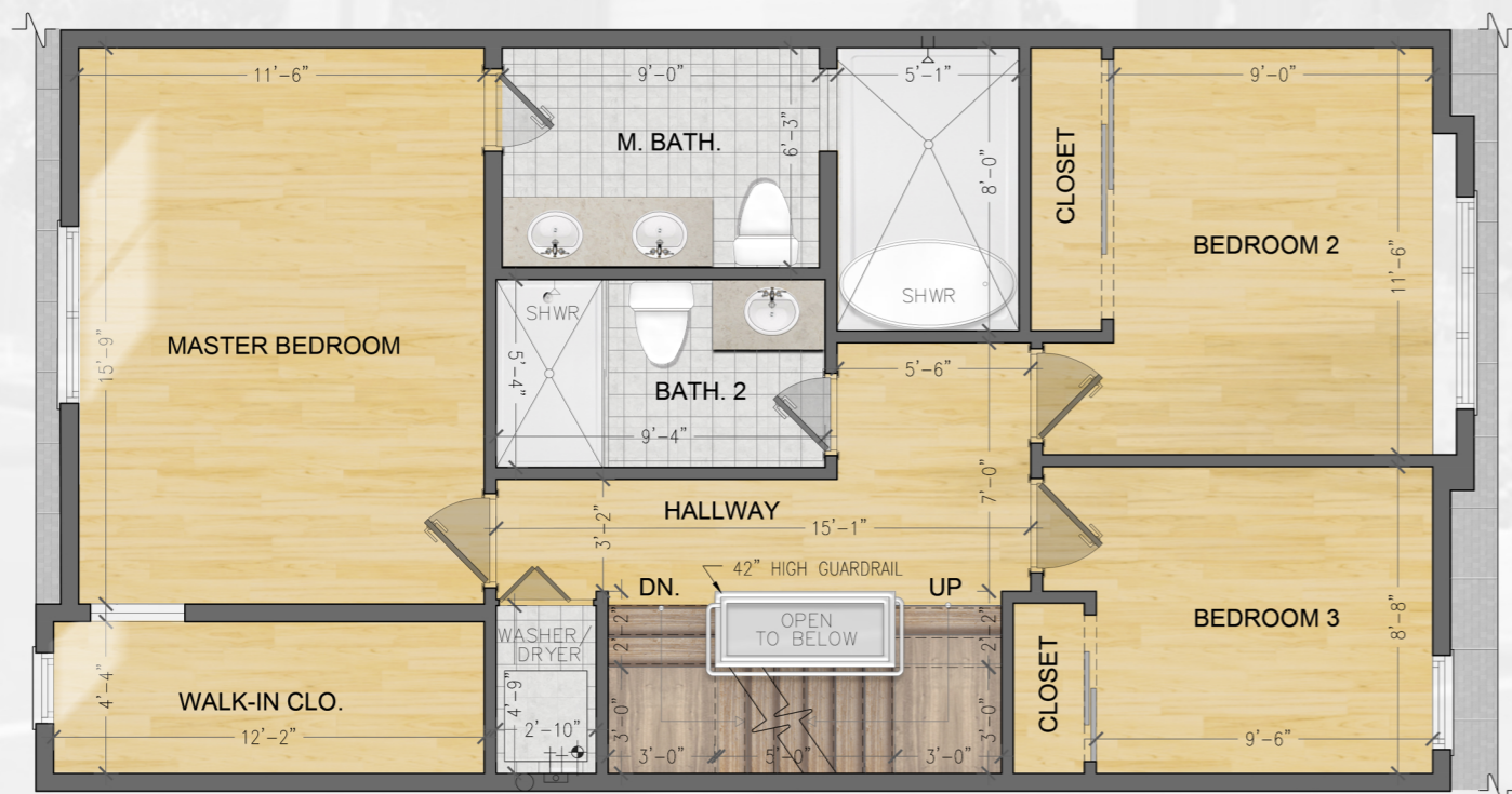
3 THIRD FLOOR PLAN EAST BUILDING
