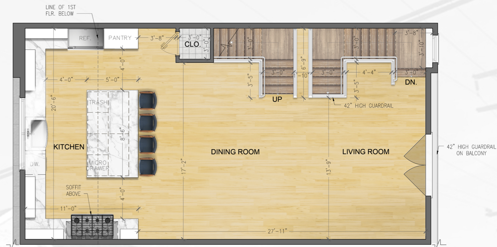
2 SECOND FLOOR PLAN EAST BUILDING
