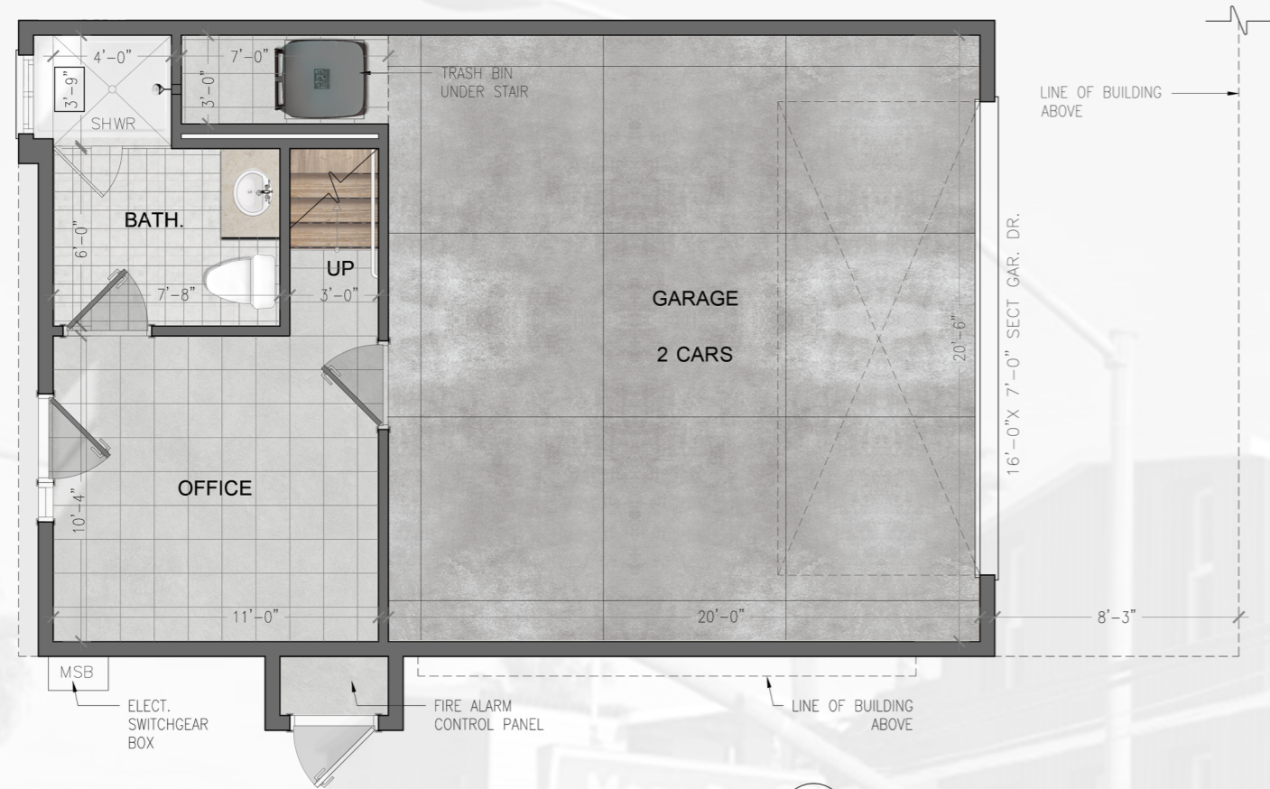
1 FIRST FLOOR PLAN WEST BUILDING
