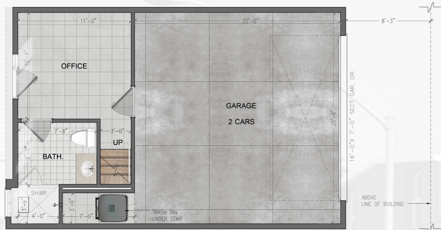
1 FIRST FLOOR PLAN WEST BUILDING
