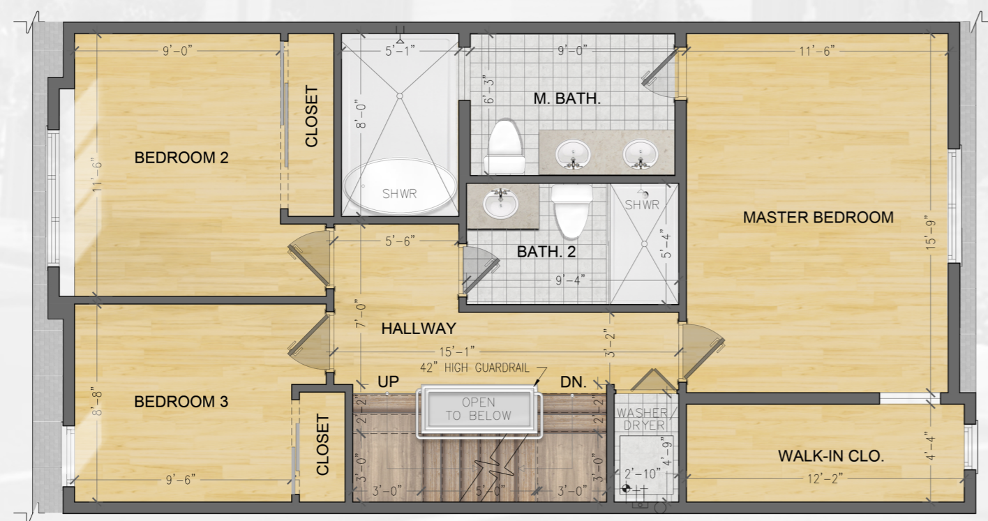
3 THIRD FLOOR PLAN WEST BUILDING
