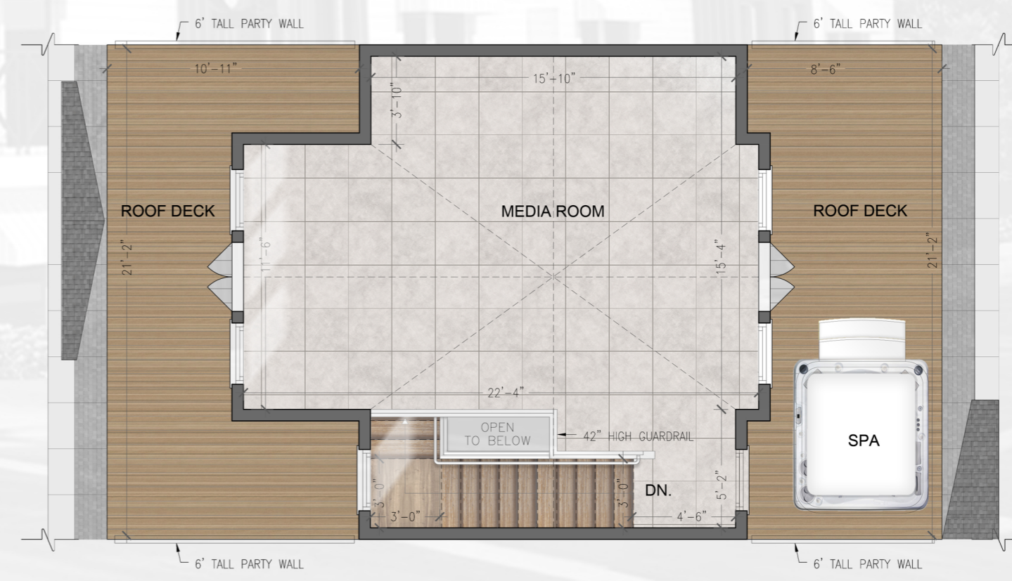
4 FOURTH FLOOR PLAN WEST BUILDING
