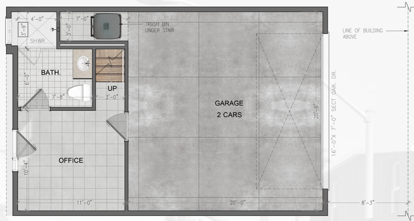
1 FIRST FLOOR PLAN WEST BUILDING
