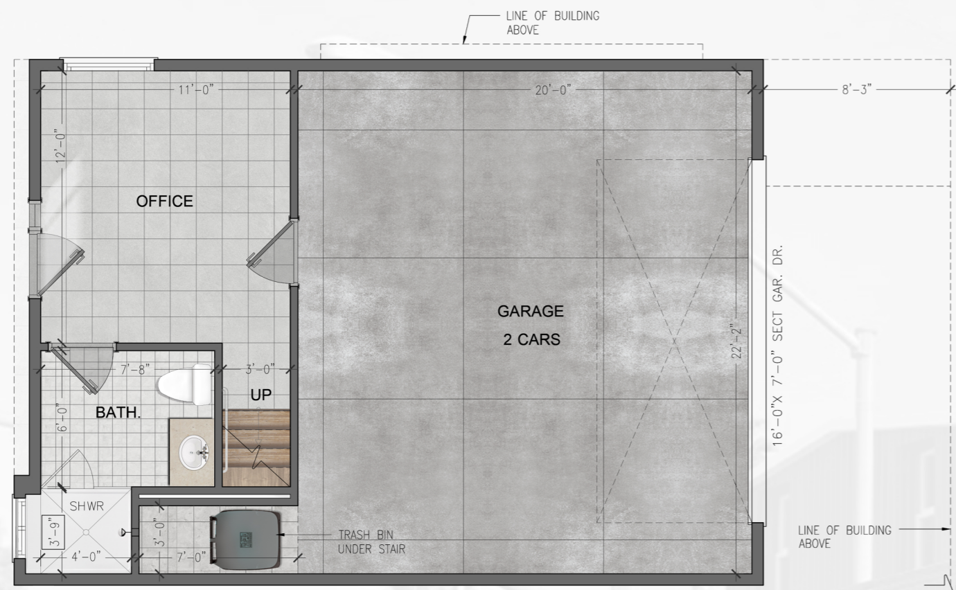
1 FIRST FLOOR PLAN WEST BUILDING
